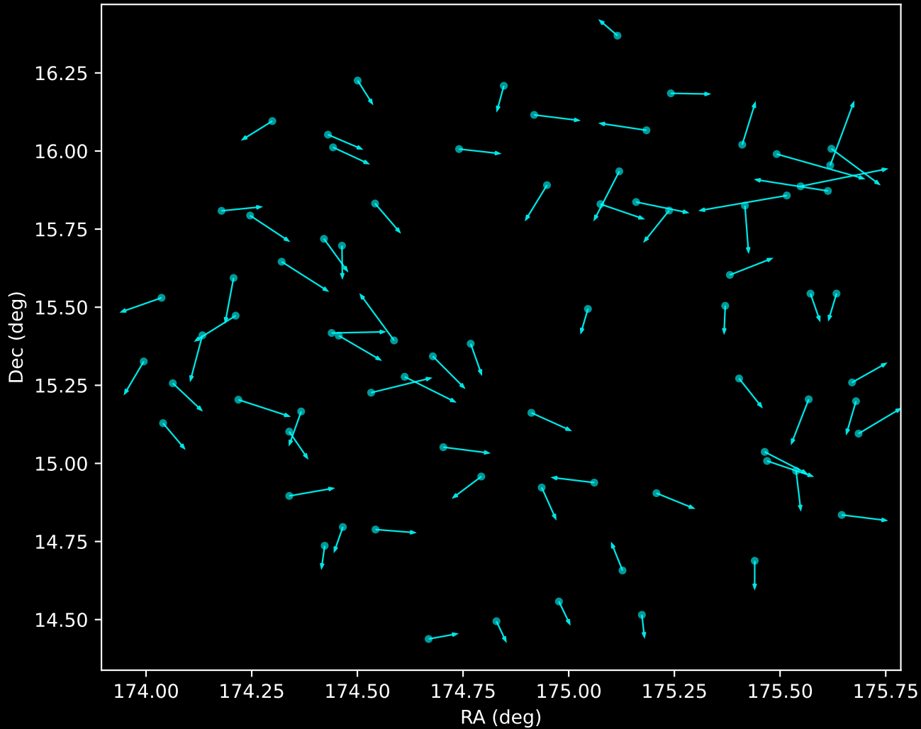
GALAH DR4 Noise Stream Proper Motion Vectors (n=76)
