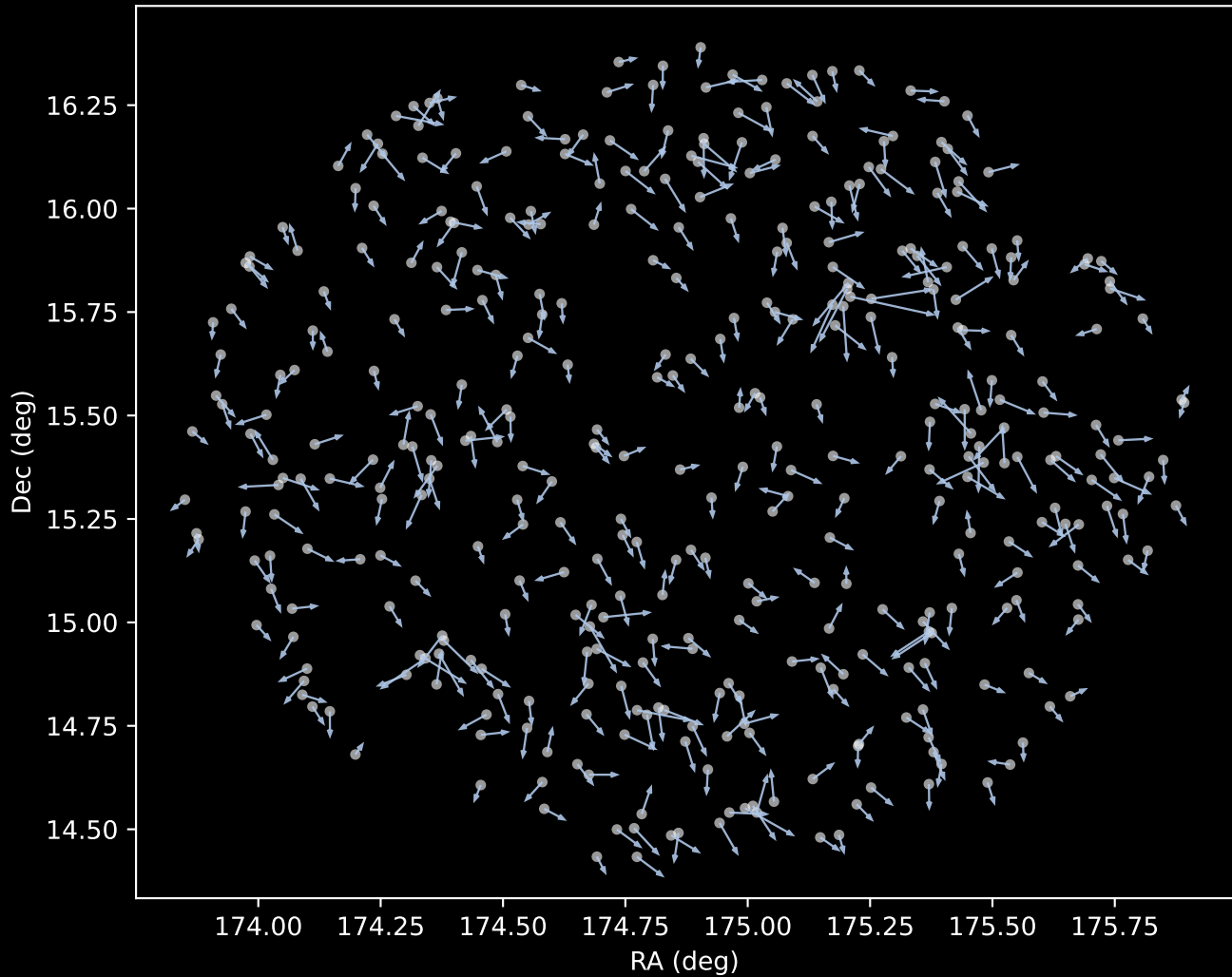
GALAH DR4 Cluster 1 Proper Motion Vectors (n=388)
