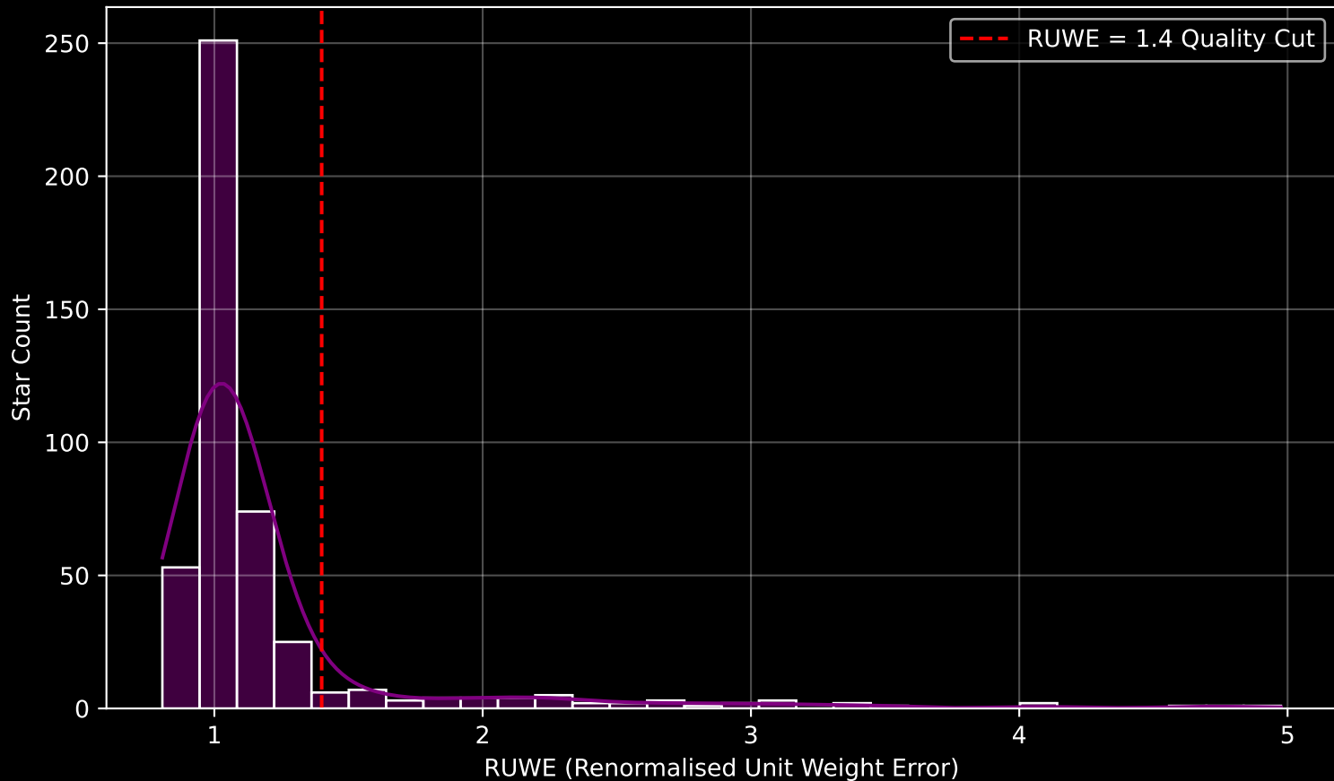
GALAH DR4 Field [6780] RUWE Distribution (n= 457)
