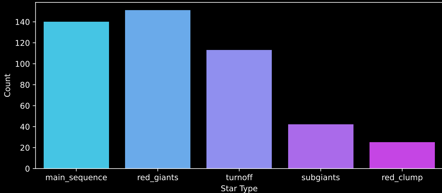
GALAH DR4 Field: [6780] Count plot of Star Type
